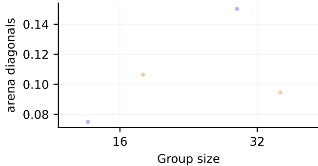
Predator distance
