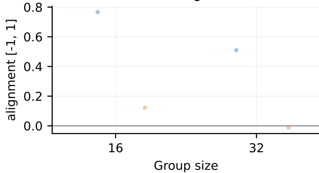
Pursuit alignment
